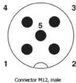
Connector M12, male
